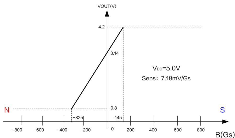
Figure5. Output characteristic curve of XL41 ( V_{DD}=5.0V )
