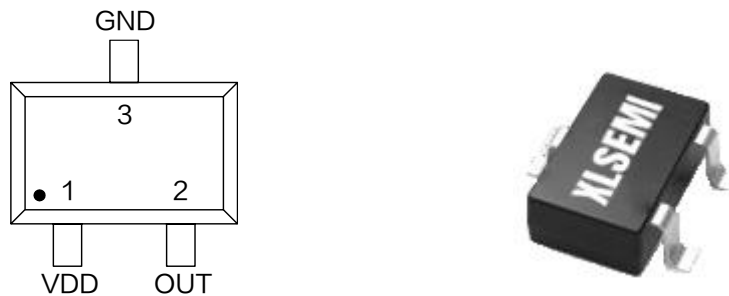
Figure2. Pin Configuration of XL41
