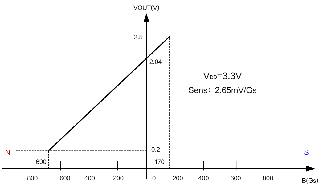
Figure 5. XL42X Output characteristic curve ( V_{DD}=3.3\text{V} )
