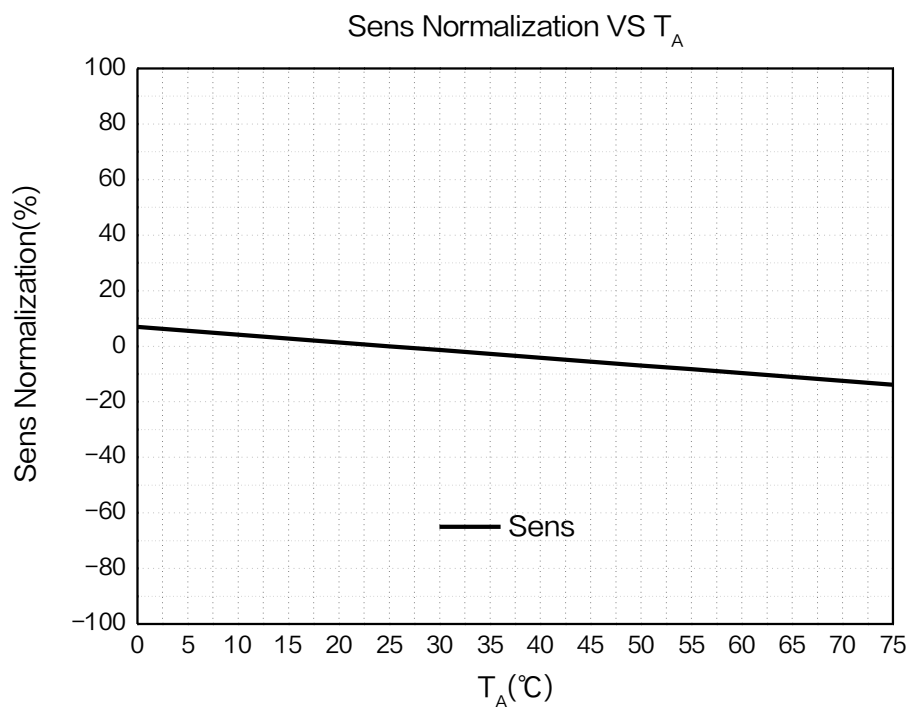
Figure6. Sensitivity versus temperature curve of XL42X ( V_{DD}=3.3V )
