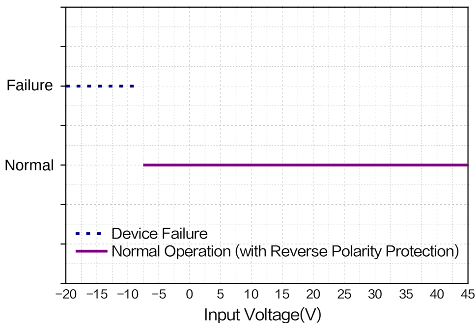
Figure 6. Input Reverse Polarity Protection Characteristic Curve of XL47E ( V_{DD} = -7.5 \sim 45V )
