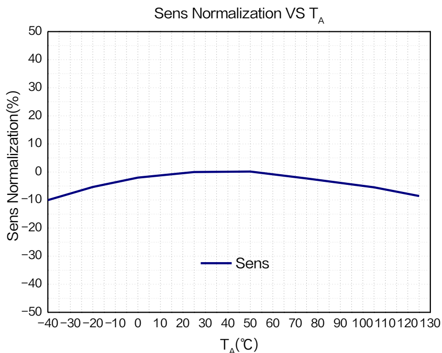
Figure 8. Sensitivity versus temperature curve of XL47E ( V_{DD} = 5.0V )
