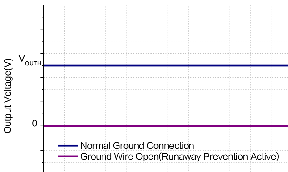
Figure 7. Runaway Prevention Function Characteristic Curve of XL47E ( V_{DD} = 5.0V )
