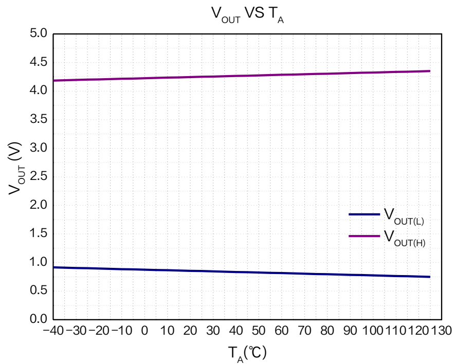
Figure 10. Output High/Low Level Temperature Characteristic Curve of XL47E
