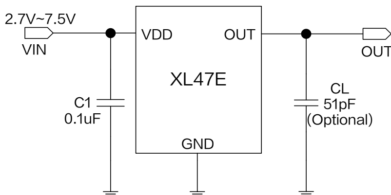
Figure1.XL47E Typical application schematic
