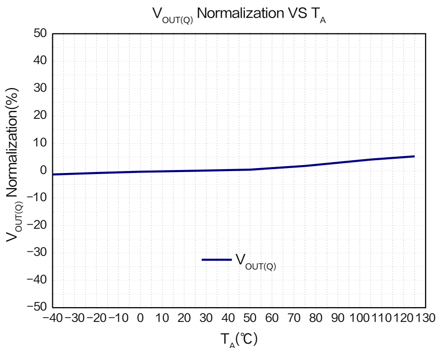
Figure 9. Static output voltage versus temperature curve of XL47E ( V_{DD} = 5.0V )
