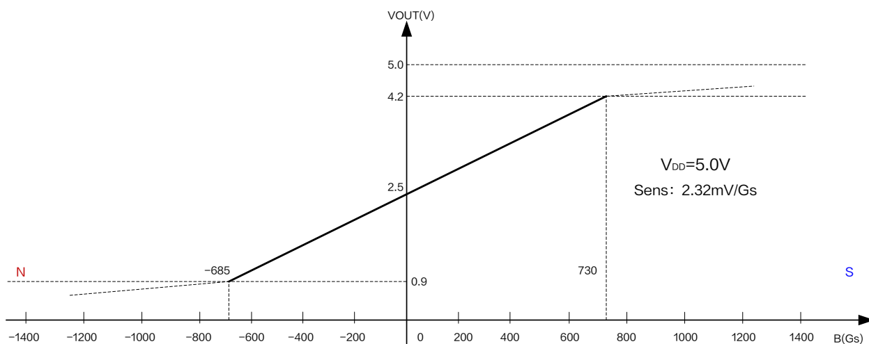
Figure5. Output Characteristic Curve of XL47E ( V_{DD} = 5.0\text{V} )
