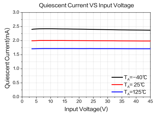
Figure 6. Quiescent Current
