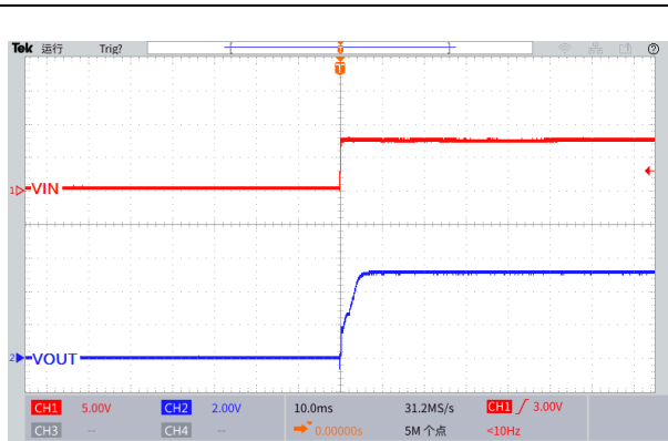
Figure 20. Start-Up Characteristic ( V_{IN}=8V , V_{OUT}=5.0V , I_{OUT}=0.1A )
