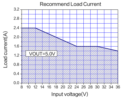
图 17.最大输出电流 ( V OUT =5.0V, T A =25°C )
