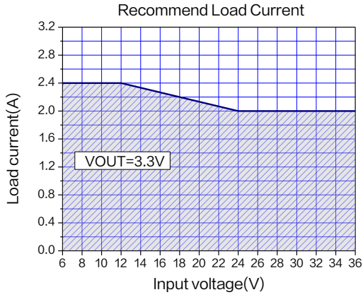
图 16.最大输出电流 ( V OUT =3.3V, T A =25°C )
