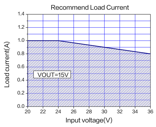
图 19.最大输出电流 ( V OUT =15V, T A =25°C )
