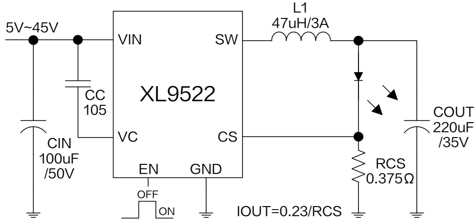
Figure6. XL9522 System Parameters Test Circuit (I OUT =0.6A)
