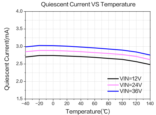
Figure16.Quiescent Current
